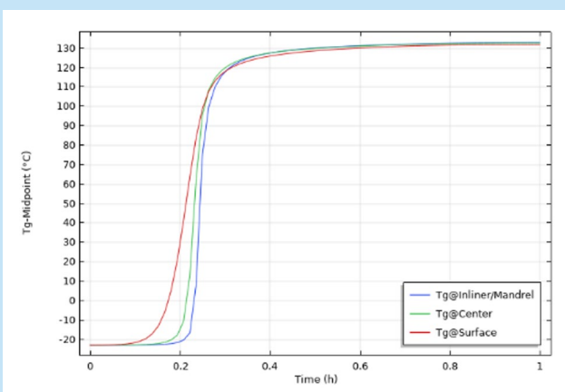
Figure 5: Tg build-up prediction for a pressure vessel cured at 150°C
