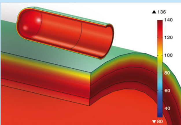
Figure 3: Temperature prediction through thickness during curing
