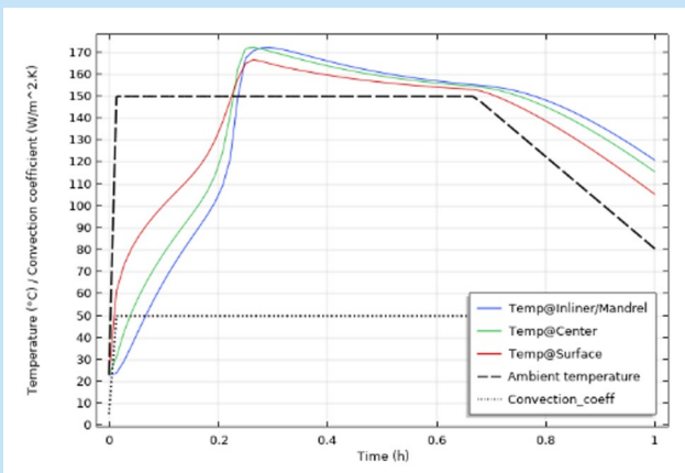
Figure 4: Temperature prediction of a pressure vessel cured at 150°C
